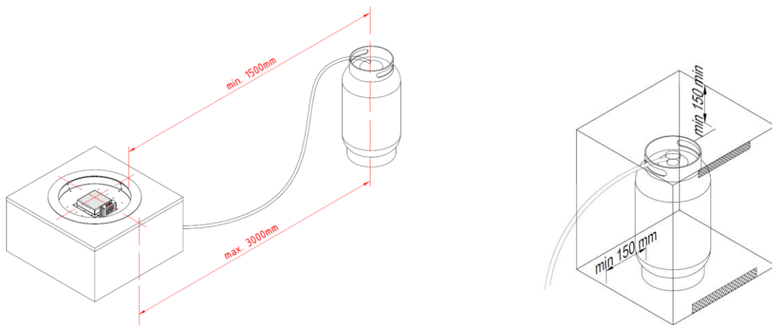
Picture 3 – Gas cylinder distance
