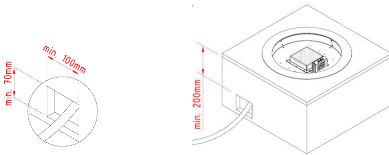
Picture 2 – Gas connection
